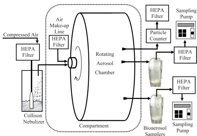
Fig. 1. Experimental setup.
